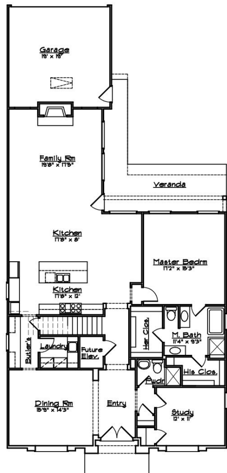
① First Floor Plan SCALE: NTS
